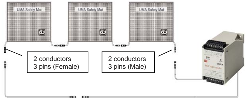
Multiple 2-Cable Mats in Series (UM□□A-□-□-2)
